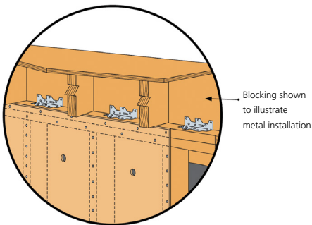
Metal framing angles connect the cripple wall to the floor system.
